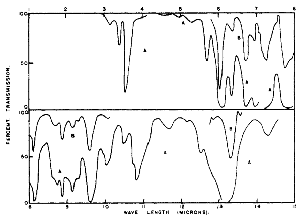
Fig. 2.—Infrared spectrogram of N-ethyl- o -ethoxyacetanilide using 0.025-mm. cell: (A) pure liquid and (B) 10% concentration in n -heptane.
